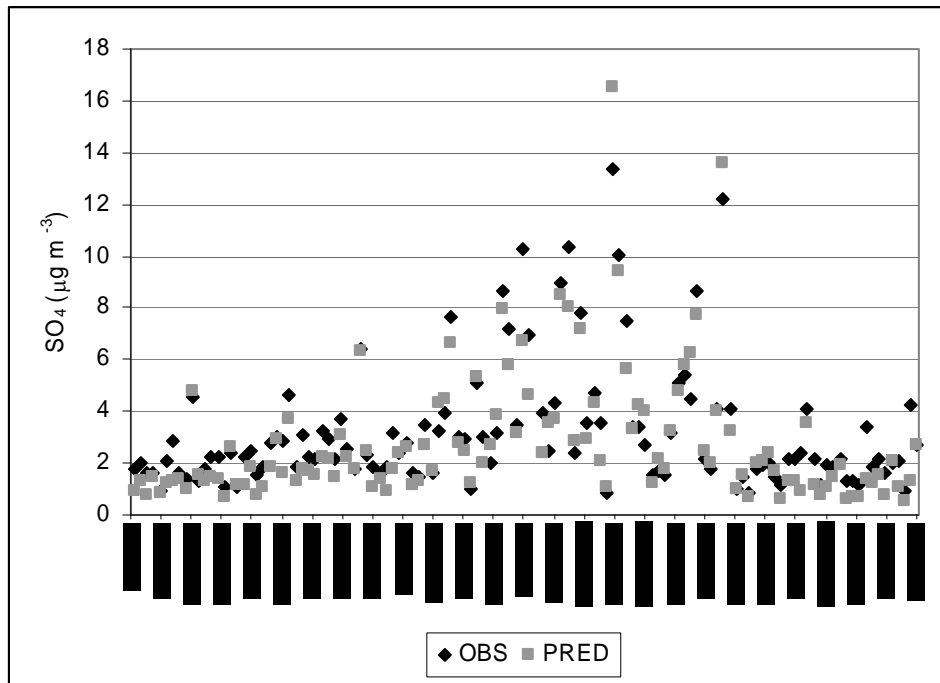
Figure 9. Time series of \text{SO}_4 mass based on the composite average of all 21 IMPROVE monitors across the OTR+ region. The observed values are denoted with the black diamonds, the model predictions are denoted with gray squares.
