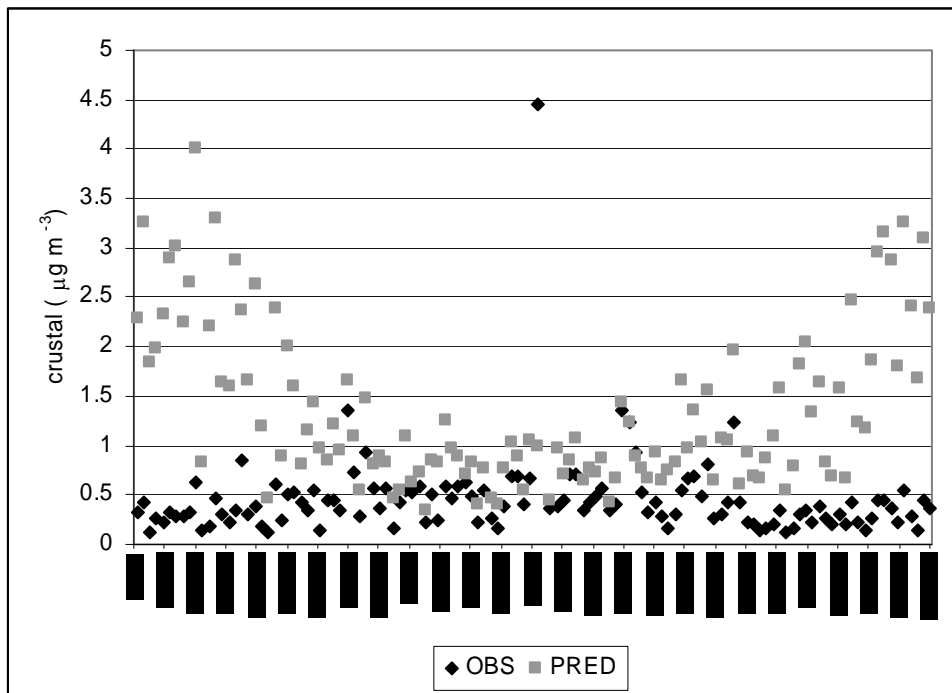
Figure 18. Time series of crustal mass based on the composite average of all 21 IMPROVE monitors across the OTR+ region. The observed values are denoted with the black diamonds, the model predictions are denoted with gray squares.
