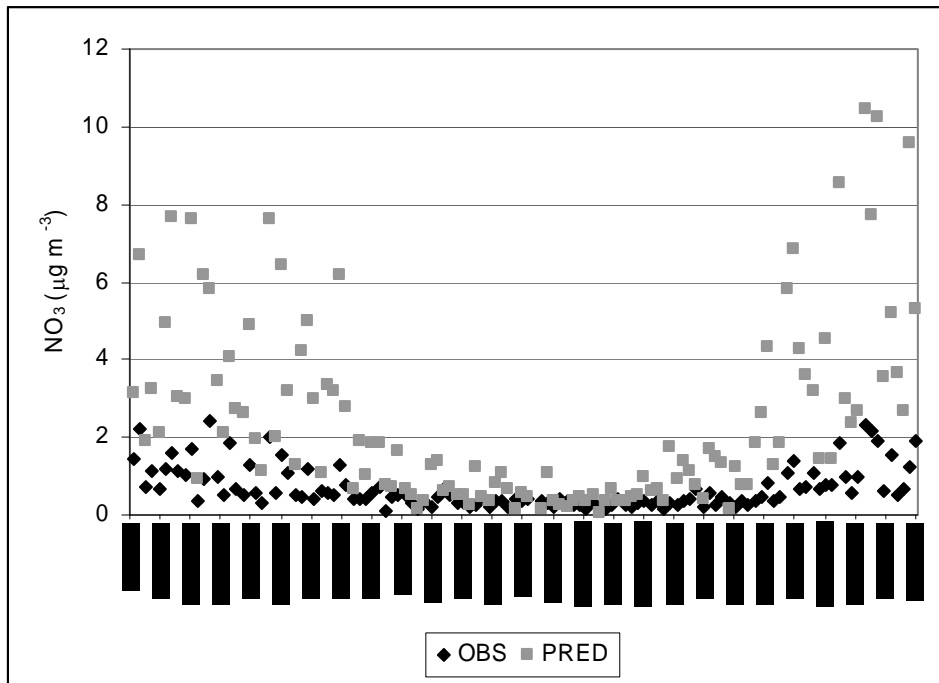
Figure 11. Time series of \text{NO}_3 mass based on the composite average of all 21 IMPROVE monitors across the OTR+ region. The observed values are denoted with the black diamonds, the model predictions are denoted with gray squares.
