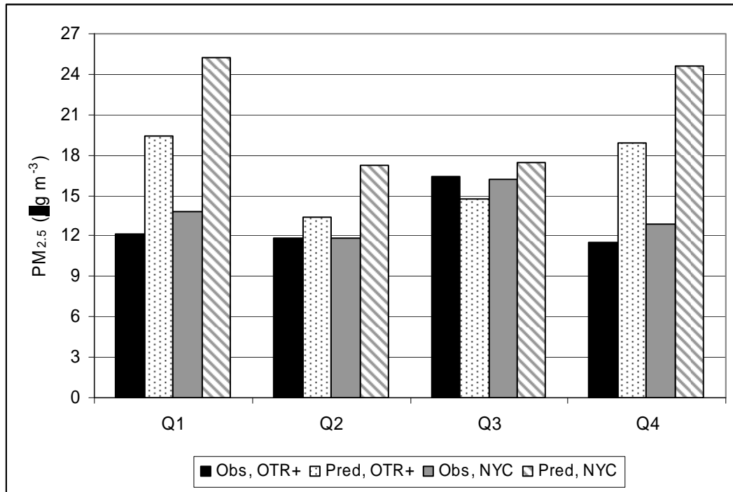
Figure 7. Observed and predicted quarterly average PM_{2.5} mass at FRM locations, for the entire OTR+ region and for the NYC NAA.
