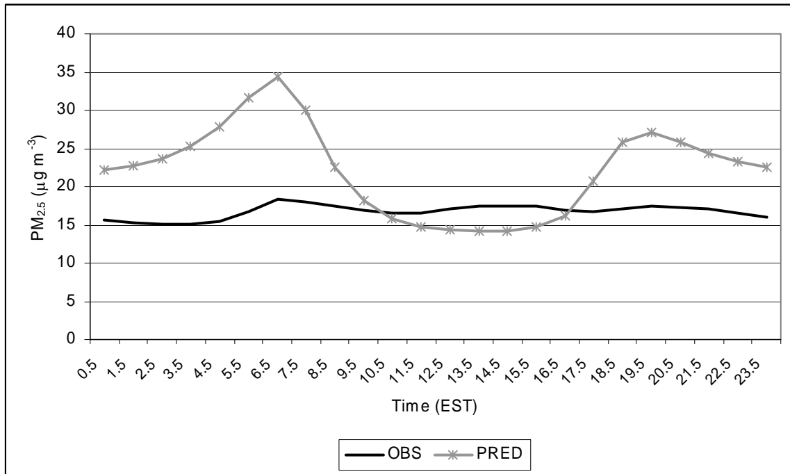
Figure 22. Composite average diurnal variation in observed (black line) and predicted (gray line) PM_{2.5} mass over the 28 hourly monitors in the NYC NAA, quarter 3.
