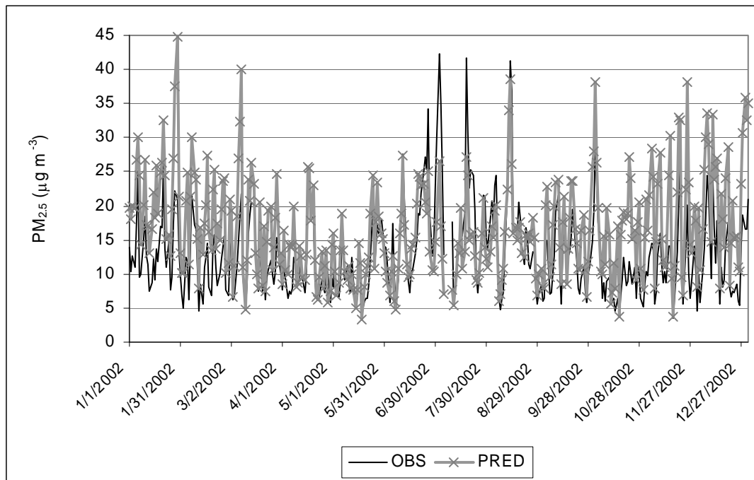
Figure 4. Time series of PM_{2.5} mass based on the composite average of all 225 FRM monitors across the OTR+ region. The observed values are denoted with the black line, the model predictions are denoted with a thick gray line and asterixes.
