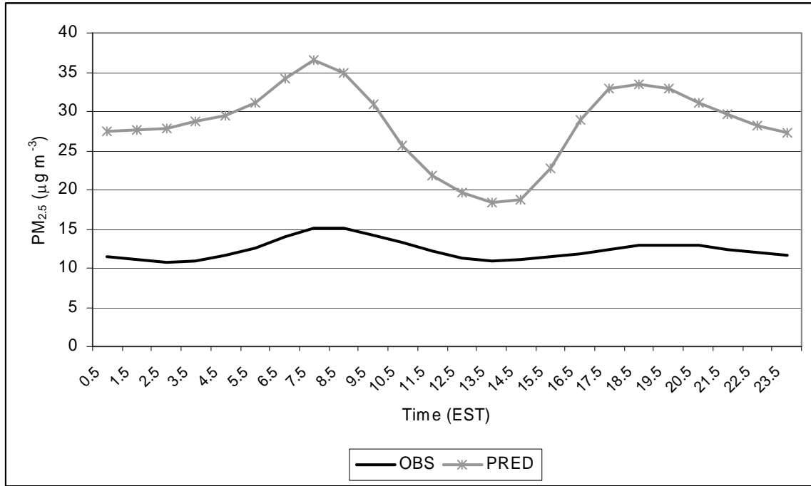
Figure 21. Composite average diurnal variation in observed (black line) and predicted (gray line) PM_{2.5} mass over the 28 hourly monitors in the NYC NAA, quarter 1.
