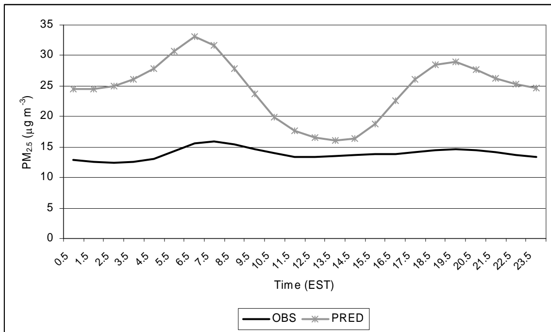
Figure 20. Composite average diurnal variation in observed (black line) and predicted (gray line) PM 2.5 mass over the 28 hourly monitors in the NYC NAA, entire year.
