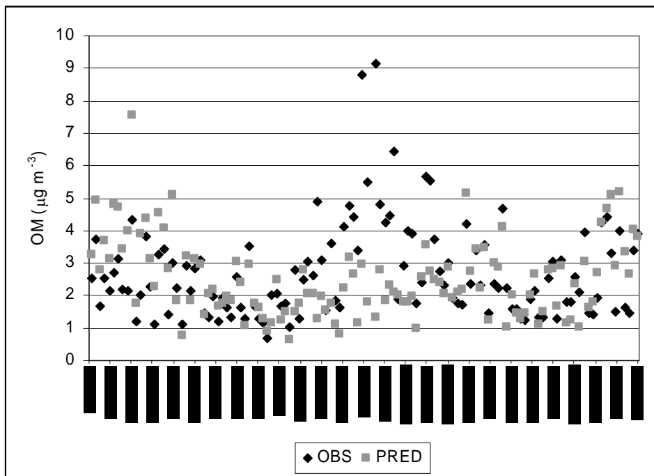
Figure 16. Time series of OM mass based on the composite average of all 21 IMPROVE monitors across the OTR+ region. The observed values are denoted with the black diamonds, the model predictions are denoted with gray squares.
