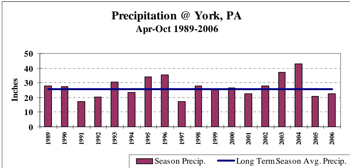
Chart 1-7 Precipitation Totals (inches) at York
