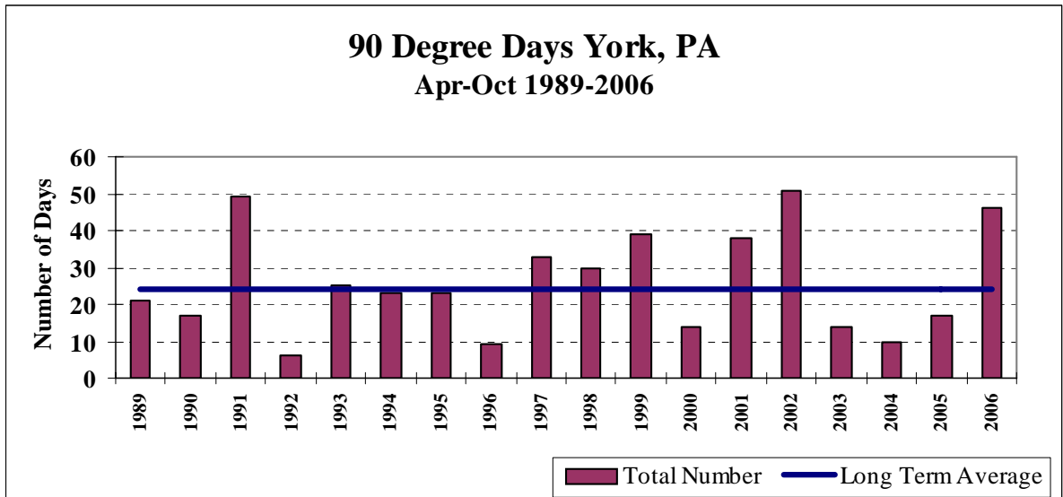
Chart 1-6 Number of 90° Degree Days at York
