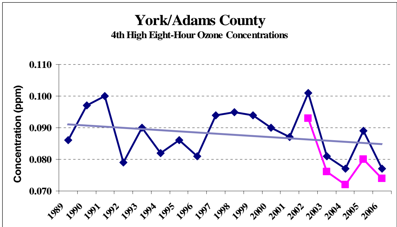
Chart 1-3 4 th High Eight-Hour Ozone Values for the York/Adams Nonattainment Area
