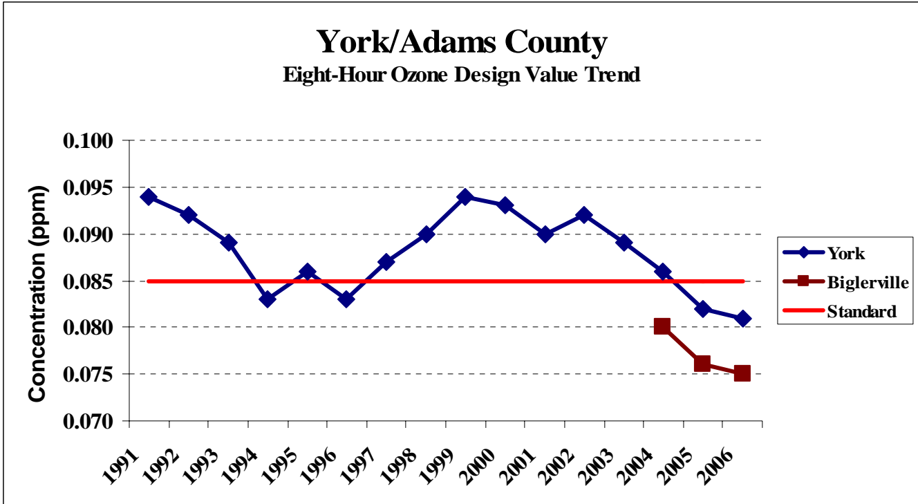
Chart 1-1 Eight-Hour Ozone Design Values
