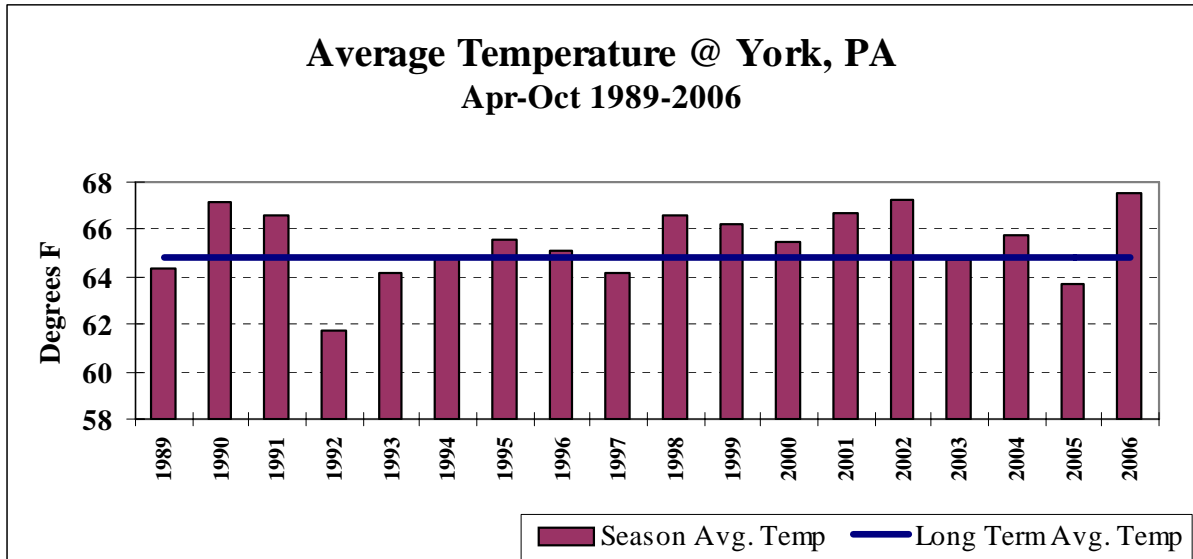
Chart 1-5 Average Temperatures at York
