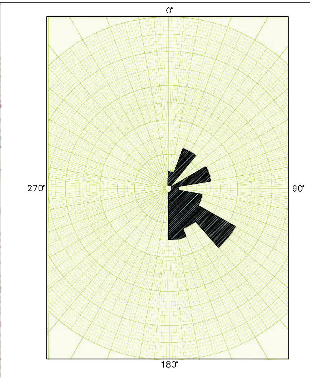
ROSE DIAGRAM LINEAMENT TRACES UNMINED AREA
