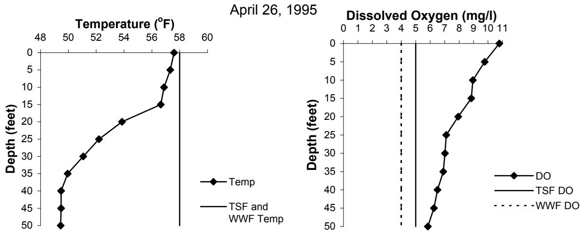
FIGURE 7. BLUE MARSH LAKE - WATER CHEMISTRY 1 Temperature and Dissolved Oxygen Profiles - BM06 COE
