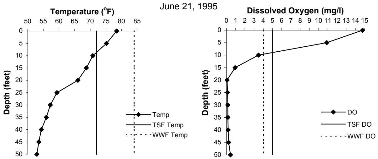
FIGURE 7. (cont.) BLUE MARSH LAKE - WATER CHEMISTRY
