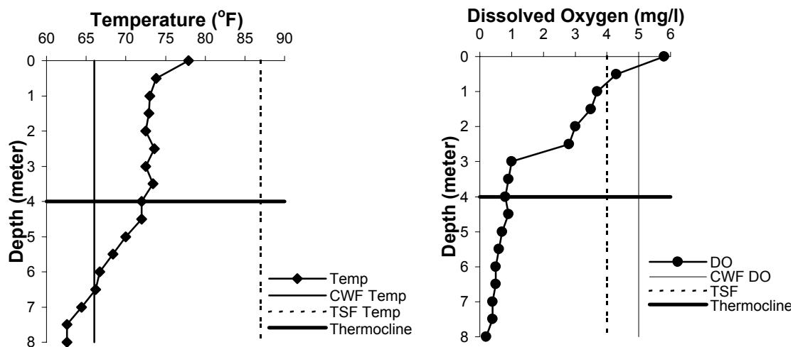
FIGURE 2. LAKE LUXEMBOURG - WATER CHEMISTRY Temperature and Dissolved Oxygen Profiles - August 26, 1985 PFBC
