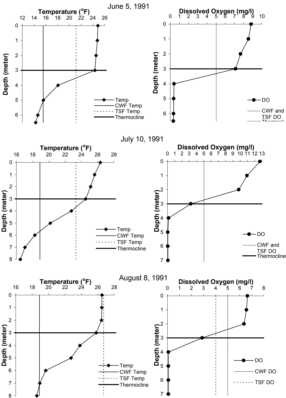
FIGURE 3. LAKE LUXEMBOURG - WATER CHEMISTRY Temperature and Dissolved Oxygen Profiles - Dam Location Coastal Vertical lines depict parameter criteria.
