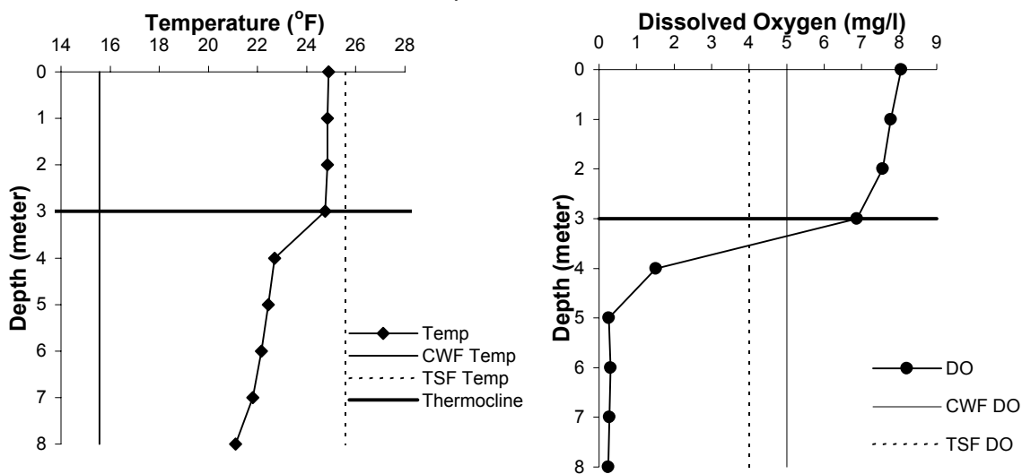
FIGURE 3. (cont.) WATER CHEMISTRY - Temperature and Dissolved Oxygen Profiles
