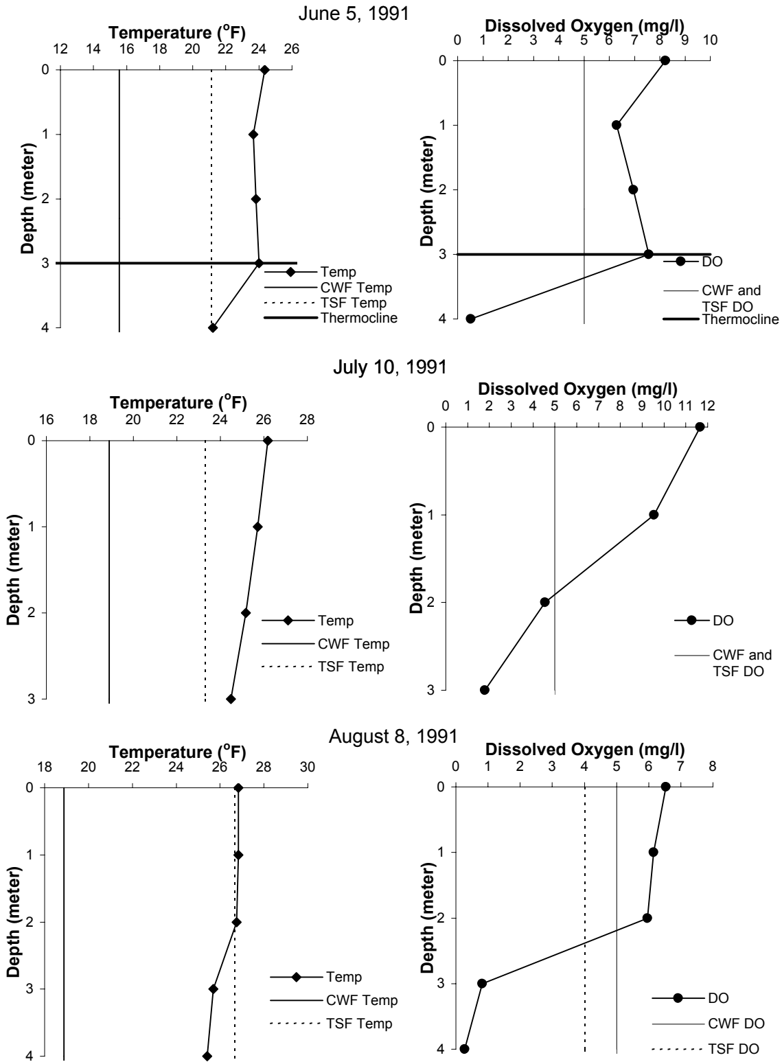
FIGURE 4. LAKE LUXEMBOURG - WATER CHEMISTRY Temperature and Dissolved Oxygen Profiles - Uplake Location Coastal Vertical lines depict parameter criteria.
